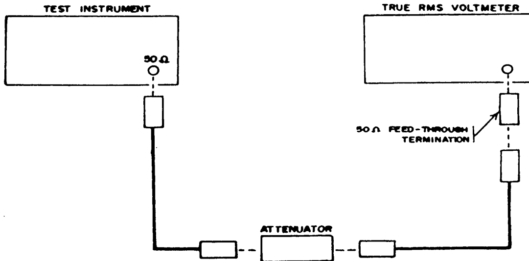
Figure 3. Output attenuator - equipment setup.
